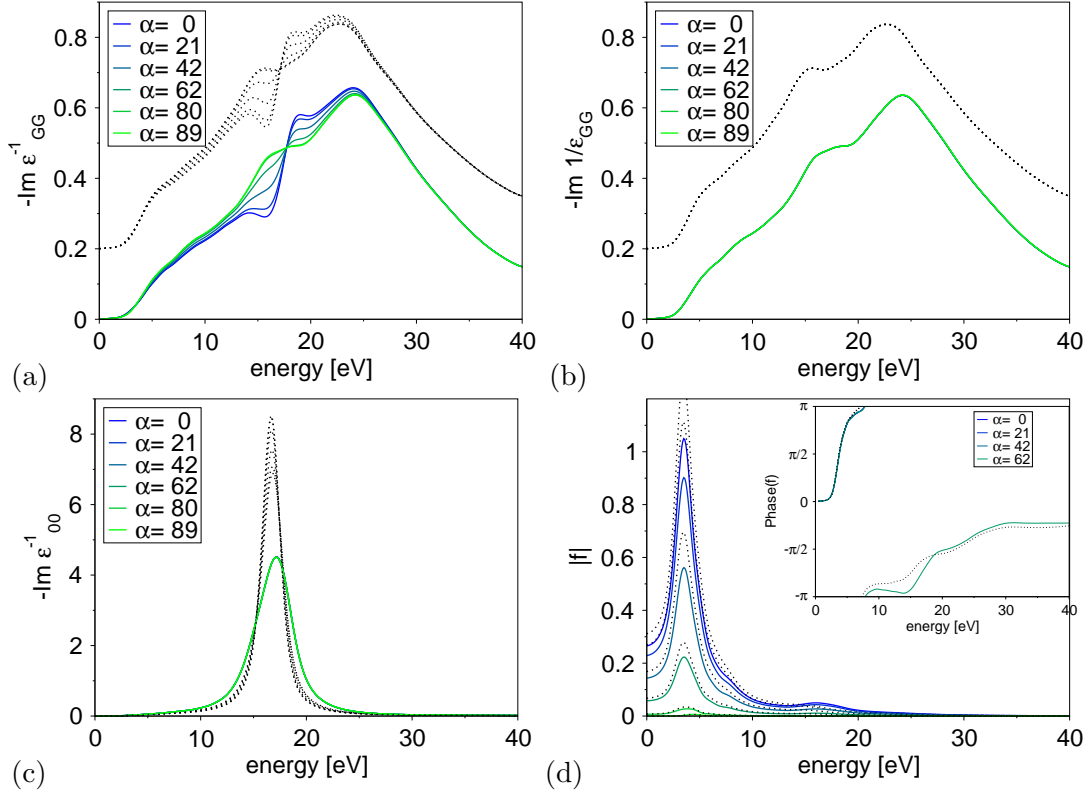
Fig. 4.8: (a) Anisotropic behaviour of the loss function -\text{Im} \varepsilon_{\mathbf{Q}\mathbf{Q}}^{-1} close to the Bragg reflection \mathbf{Q} = (1, 1, 1) in silicon. (b-d) Analysis of the contributions to the loss function following eq. (4.8). Both, results including only the \mathbf{0} and \mathbf{Q} mode (dotted lines, \varepsilon^{\text{NLF}} ) and those including all LFE are shown (solid lines, \varepsilon ). The NLF spectra in (a) and (b) are shifted along the ordinate.
