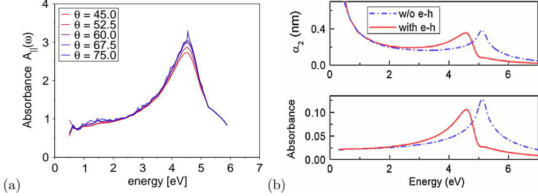
Fig. 6.15: Decomposition for the X-ray absorption measurements on isolated nanotubes of Murakami et al. [161]. We compare (a) the on-axis contribution A_{\parallel} to the absorbance of the tubes which is calculated from the experimental data shown in fig. 6.3a with (b) the absorbance of graphene obtained from a Bethe-Salpeter calculation by Yang et al. [159] (Reproduced from [159], © 2009 by The American Physical Society).
