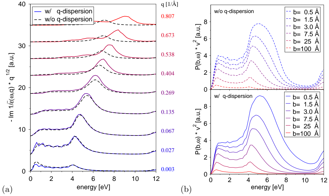
Fig. 7.2: Electron energy-loss spectra for a graphene sheet with and without nonlocal effects. (a) Angular-resolved EELS -\text{Im} \bar{\varepsilon}^{-1}(\bar{\mathbf{q}}) \propto \pi L_z v(\bar{\mathbf{q}}) S(\bar{\mathbf{q}}) for different in-plane momentum transfers \bar{q} . The spectra have been shifted along the ordinate. (b) Spatially-resolved EELS for several impact parameters b [see eq. (7.6)]. In (a) and (b), the dynamic structure factor S(\bar{\mathbf{q}}) of graphene is calculated in a local approximation [eq. (7.8), dashed] or by full ab-initio calculations (solid).
