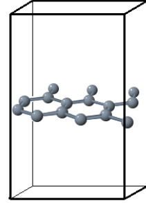
Fig. 3.3: Supercell
