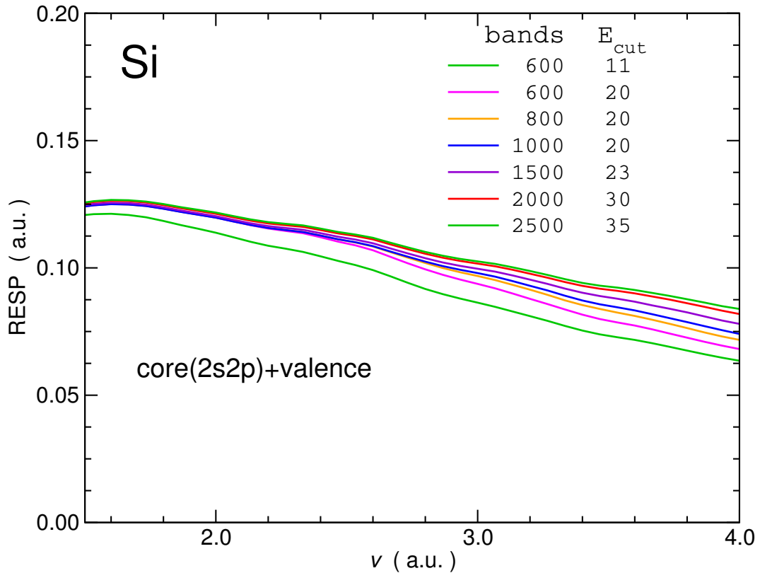
Figure 6.9: Convergence of the RESP of silicon within RPA as a function of the number of bands and of the dielectric matrix cutoff. The convergence with respect to the number of bands and dielectric matrix cutoff was obtained for a fixed \Gamma -point sampling. The convergence study is obtained for the (2s2p3s3p) electrons.
