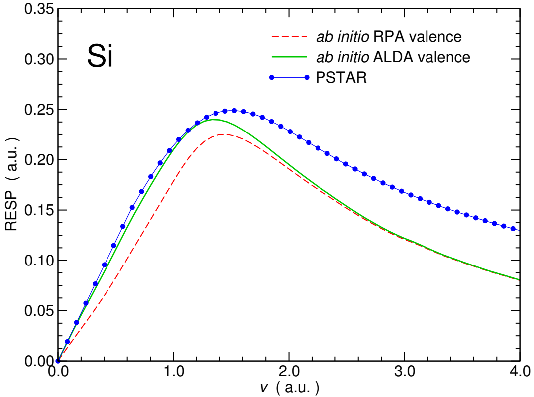
Figure 7.3: RESP of Si using different approximations for the TDDFT kernel: RPA (dashed red line) and ALDA (solid green line). Silicon is described by its valence electrons only. Experiment from the PSTAR database[7] (blue circle symbols) is given as a reference.
