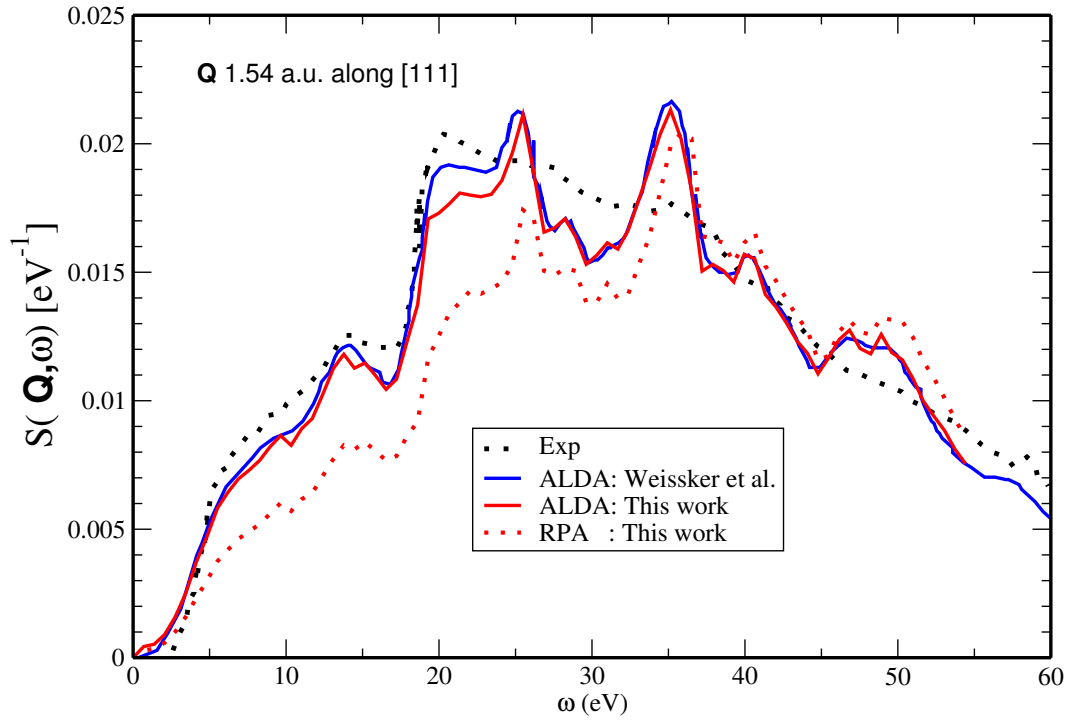
Figure 7.2: Comparison of the calculated dynamic structure factor using both RPA and ALDA with the available theoretical and experimental data for silicon. Both the experimental and theoretical data have been taken from Ref. [87]. The present results have been obtained using the same convergence parameters as found in Ref.[87].
