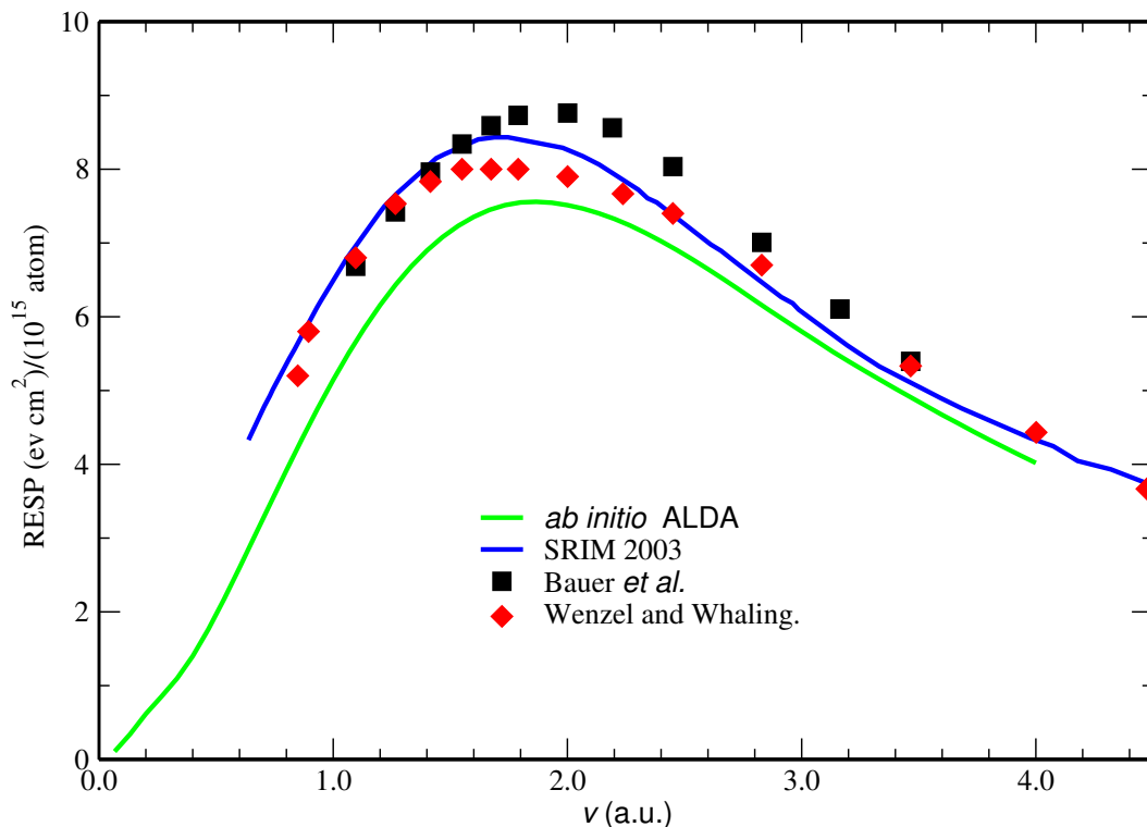
Figure 8.2: The validity of RESP of plane wave framework in evaluating of ice-Ih target within ALDA in linear-response (solid green line) compared to the available experimental data. Experiments by Bauer et al. [5] (black square points) and Wenzel and Whaling [89] (red diamond points). The SRIM 2003 [93] is semi empirical code (solid blue line).
