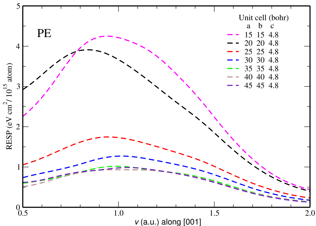
Figure 8.8: Volume convergence test of PE. RESP of proton in the PE target as a function of the cell volume V_c (The cell is orthorhombic P type). For all V_c the following parameters have been used: N_k = 1 the gamma point, E_{cut} = 8 Ha for \epsilon_{\mathbf{G}\mathbf{G}'}^{-1}(\mathbf{q}, \omega) , \eta = 6 eV and using \Delta E_{band} = 68 eV energy band. The same excitation density is used for the all V_c .
