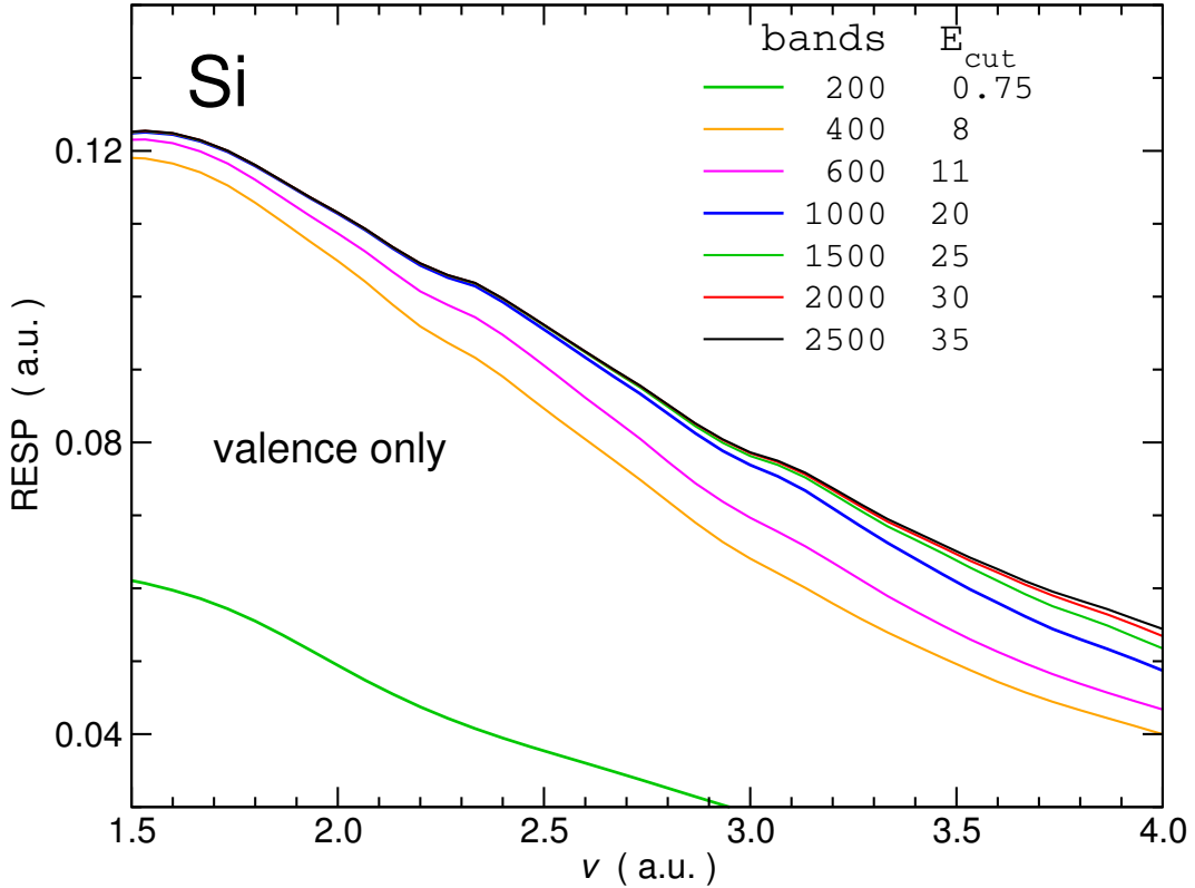
Figure 6.5: Convergence of the RESP of silicon within RPA as a function of the number of bands and of the dielectric matrix cutoff. The convergence with respect to the number of bands and dielectric matrix cutoff was obtained at a fixed \Gamma -point sampling.
