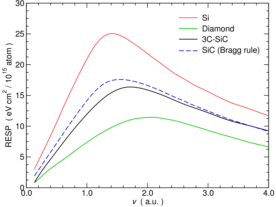
Figure 7.9: RESP of Si, diamond, 3C-SiC within ALDA including the 2s2p electrons of Si. The Bragg's rule SiC (dashed blue line) was obtained using Eq. (7.3).
