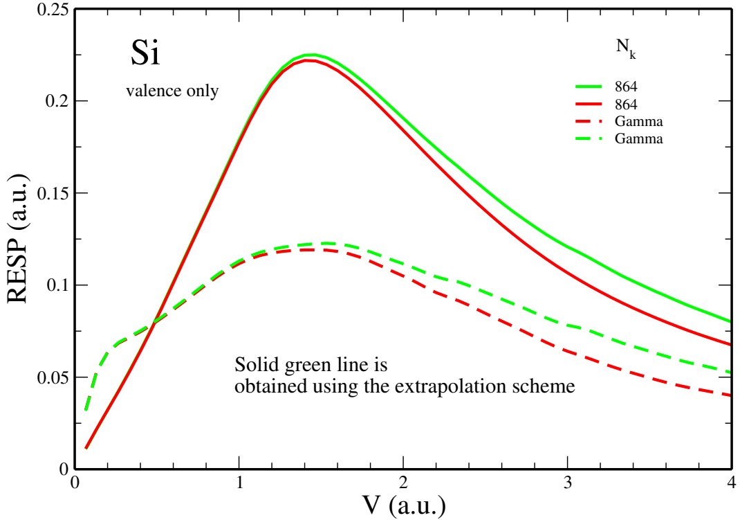
Figure 6.8: The fully Converged RESP of valence electrons in Si target for proton ( Z_1=1 ) within the linear response of RPA calculated by extrapolation scheme in Eq. (6.4). The green line obtained for highly converged parameters (2000 bands and E_{cut} = 25 Ha), the red line obtained for low converged parameters (400 bands and E_{cut} = 8 Ha).
