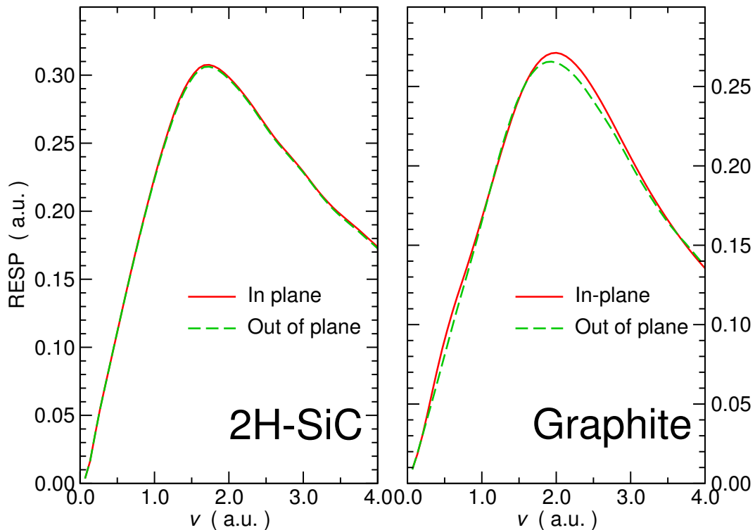
Figure 7.8: Anisotropy of the RESP of 2H-SiC (left-hand panel) and of graphite (right-hand panel) within ALDA including the 2s2p electrons of Si.
