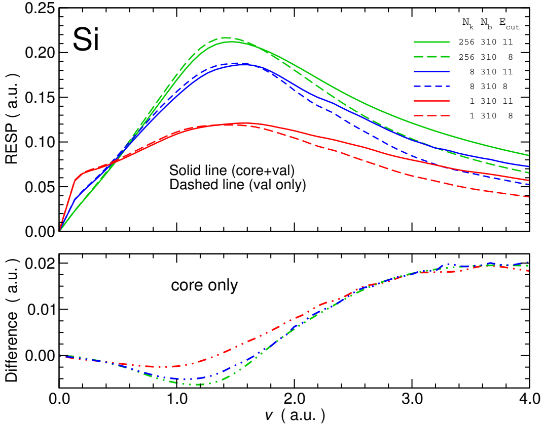
Figure 6.7: Comparison of the RESP core contribution calculated using 3 \mathbf{k} -point meshes: 256 BZ points (green lines), 8 BZ points (blue lines) and \Gamma (red lines). The upper panel shows the RESP for two levels of electrons contribution, i.e., the 2s2p3s3p electrons and 3s3p electrons only whereas the lower panel shows their difference, i.e., the 2s2p electrons only).
