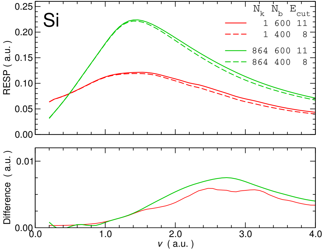
Figure 6.6: Comparison of the convergence rate for 2 \mathbf{k} -point meshes: \Gamma (red lines) and 864 BZ points (green lines). The upper panel shows the RESP for two levels of convergence, whereas the lower panel shows their difference.
