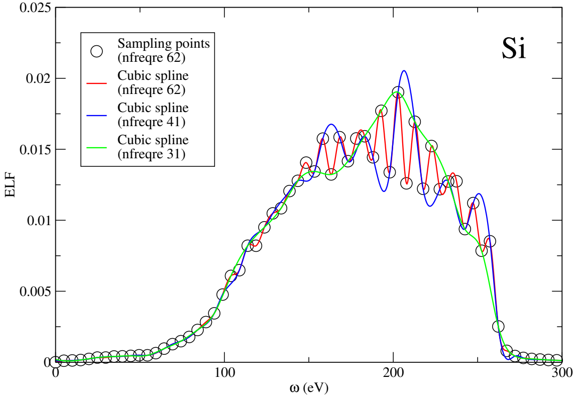
Figure 6.2: The accuracy of using the cubic spline interpolation with increasing the nfreqre . All the calculated values are obtained at |\mathbf{q} + \mathbf{G}| = 3.71 a.u. along [111] . This study have been done using the following parameters: 4 \times 4 \times 4 with 4 shifts of \mathbf{q} point mesh, 400 bands and the broadening \eta is 1.5 eV.
