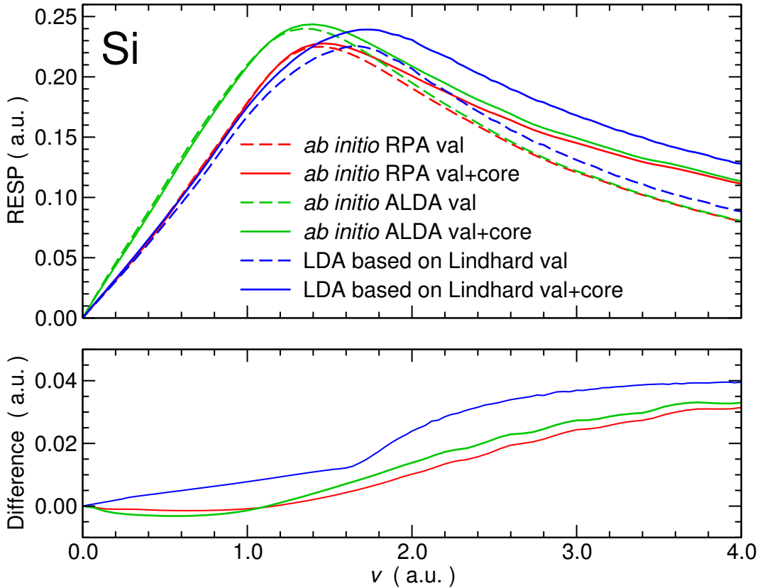
Figure 7.5: Upper panel: RESP of Si within RPA (red lines), ALDA (green lines), and LDA based on Lindhard (blue lines) including (solid lines) or not (dashed lines) the contribution from the core 2s and 2p electrons. Lower panel: Core-only contribution to the RESP of Si as obtained through the difference between the calculations with and without 2s and 2p within RPA, ALDA, or LDA based on Lindhard.
