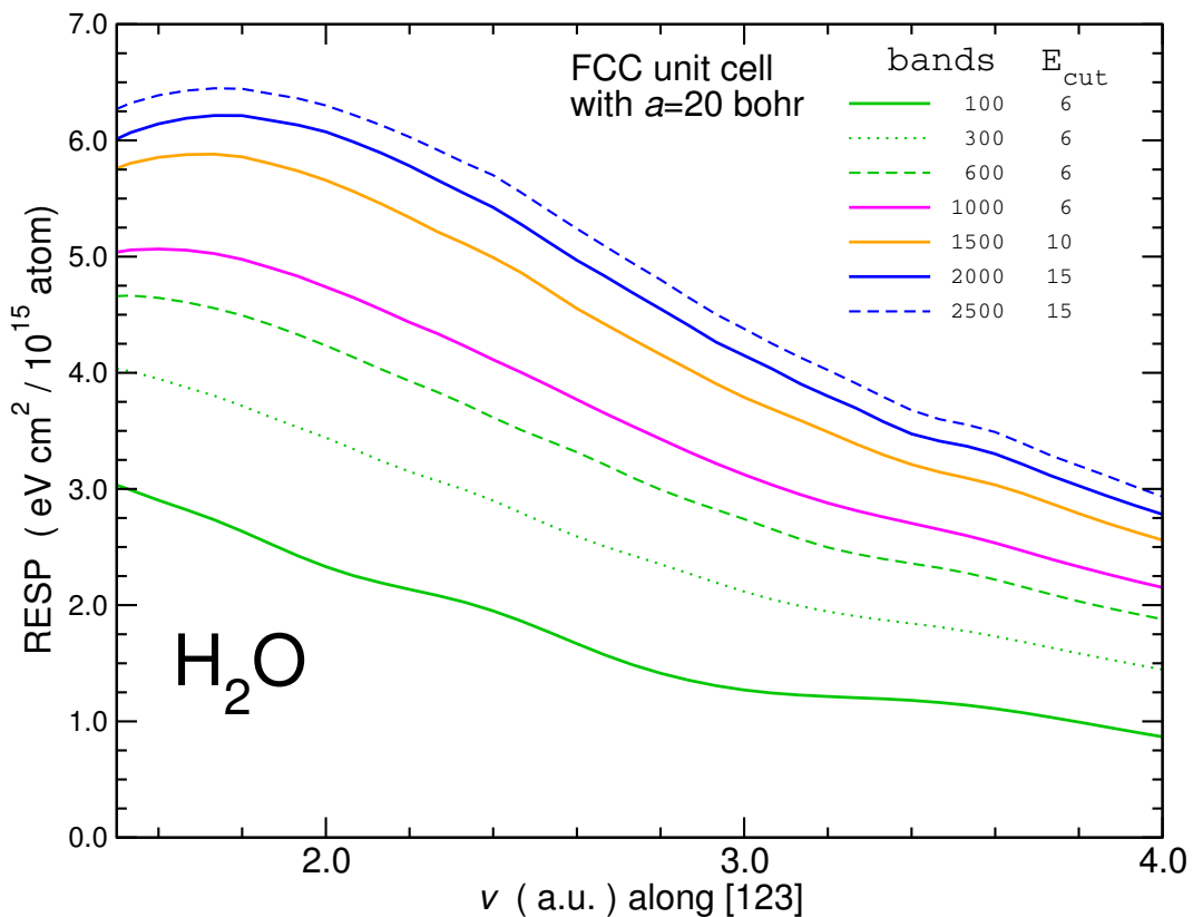
Figure 8.4: Convergence of the RESP of H_2O gas target within ALDA as a function of the number of bands and of the dielectric matrix cutoff. The convergence with respect to the number of bands and dielectric matrix cutoff was obtained for a fixed \Gamma -point sampling with \eta = 4 eV. The convergence study is obtained for the all electrons (without 1s state of the oxygen atom).
