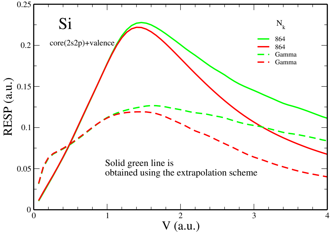
Figure 6.10: The fully Converged RESP of (2s2p3s3p) electrons in Si target for proton ( Z_1=1 ) within the linear response of RPA calculated by extrapolation scheme in Eq. (6.5). The green line obtained for highly converged parameters (2500 bands and E_{cut} = 35 Ha) for the all electrons (without 1s), the red line obtained for low converged parameters (400 bands and E_{cut} = 8 Ha) for valence only.
