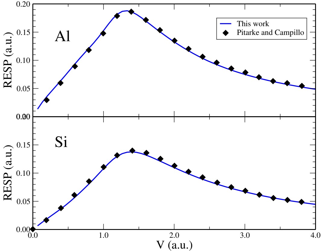
Figure 6.3: Comparison of the RESP as a function of the projectile velocity within RPA from our implementation (solid blue line) against previously published results from Ref. [64] (black diamond symbols). The calculations are converged with the same level of accuracy as prescribed in the previous work.
