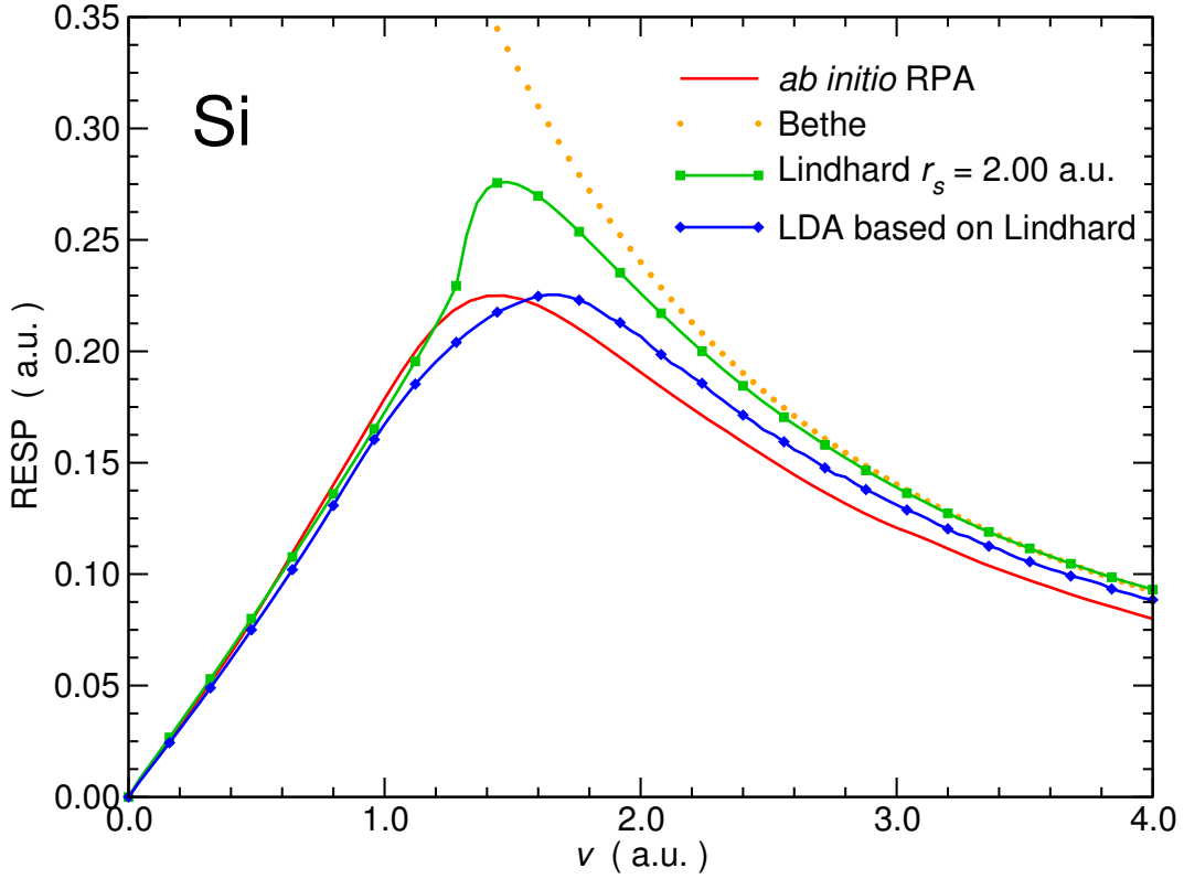
Figure 7.1: FEG-based modeling of the RESP against the reference ab initio RPA calculation.
