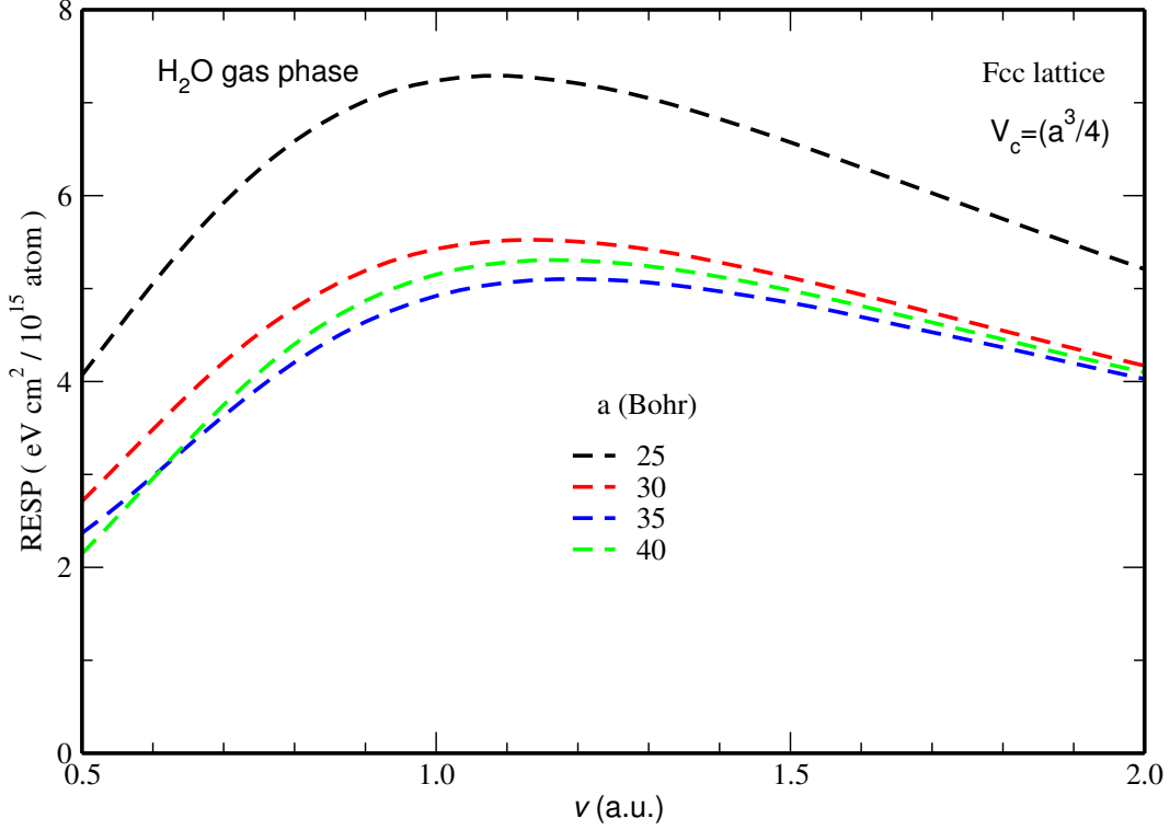
Figure 8.3: RESP of proton in the H 2 O gas phase target as a function of the cell volume V_c . For all V_c the following parameters have been used: N_k = 8 , E_{cut} = 4 Ha for \varepsilon_{\mathbf{G}\mathbf{G}'}^{-1}(\mathbf{q}, \omega) , \eta = 1.5 eV and using a number of bands so that the highest transition is \Delta E_{band} = 42 eV. Thus, the same excitation density will be used for all the volume V_c . Note that the low velocity part below 0.5 a.u. is very unstable and is not shown here.
