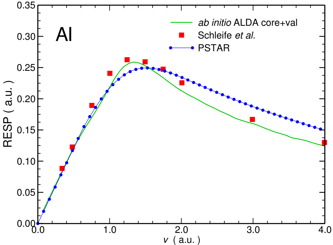
Figure 7.7: RESP of Al within ALDA in linear-response (solid green line) compared to the time-propagation results of Scheife and coauthors.[77] Experiment from the PSTAR database[7] (blue circle symbols) is given as a reference.
