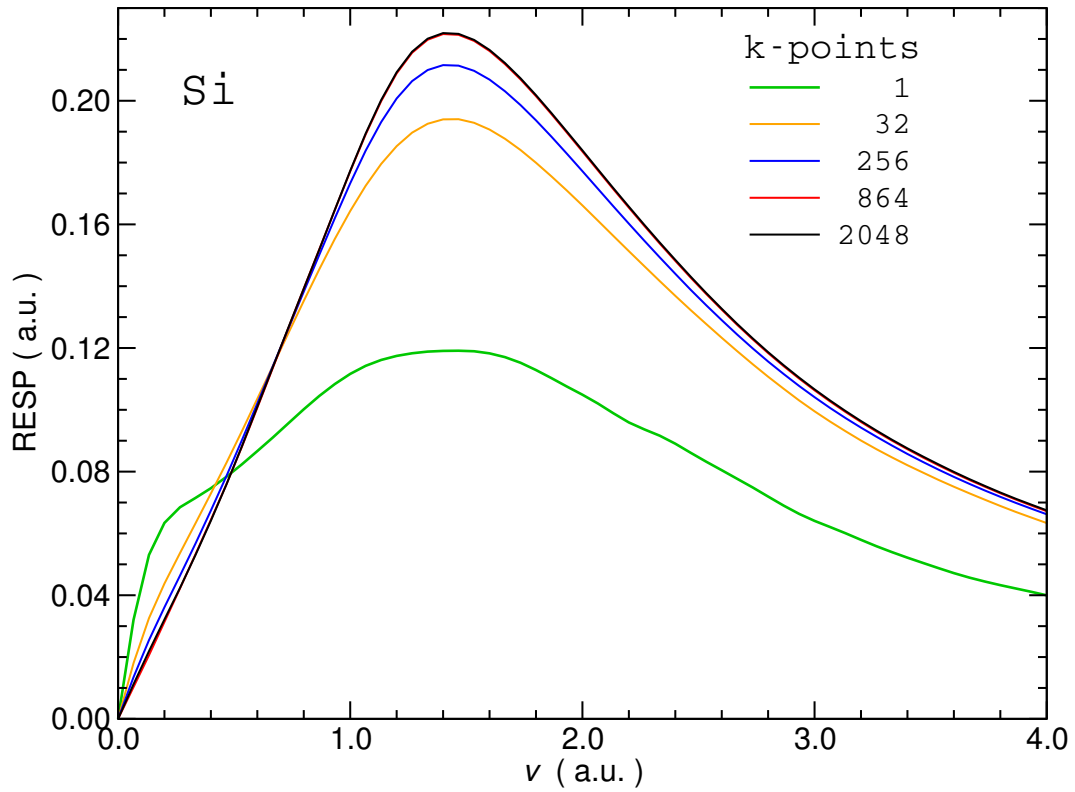
Figure 6.4: Convergence of the RESP of silicon within RPA as a function of \mathbf{k} -points. The convergence with respect to the \mathbf{k} -point grid was evaluated for a fixed number of bands (400) and a fixed dielectric matrix cutoff (8 Ha).
