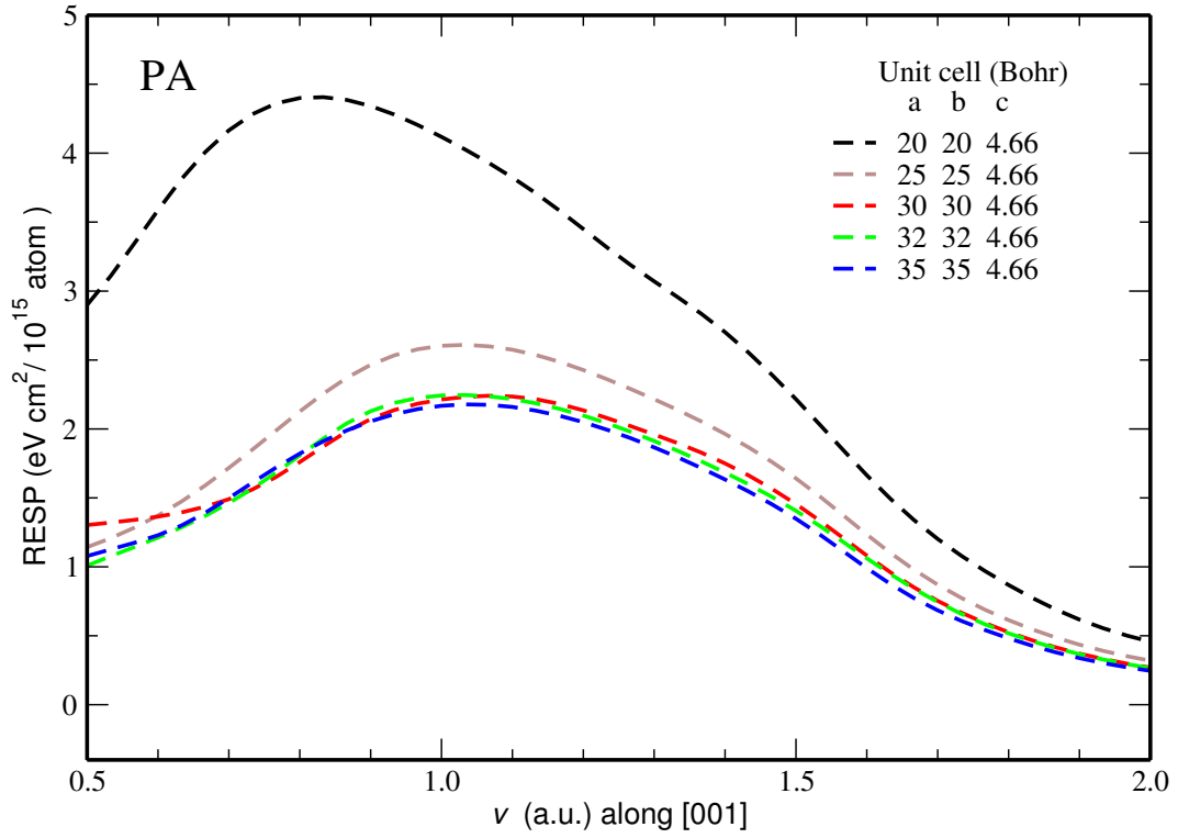
Figure 8.7: Volume convergence test of PA. RESP of proton in the PA target as a function of the cell volume V_c (The cell is orthorhombic P type). For all V_c the following parameters have been used: N_k = 1 the gamma point, E_{cut} = 8 Ha for \epsilon_{\mathbf{G}\mathbf{G}'}^{-1}(\mathbf{q}, \omega) , \eta = 6 eV and using \Delta E_{band} = 68 eV energy band. The same excitation density is used for the all V_c .
