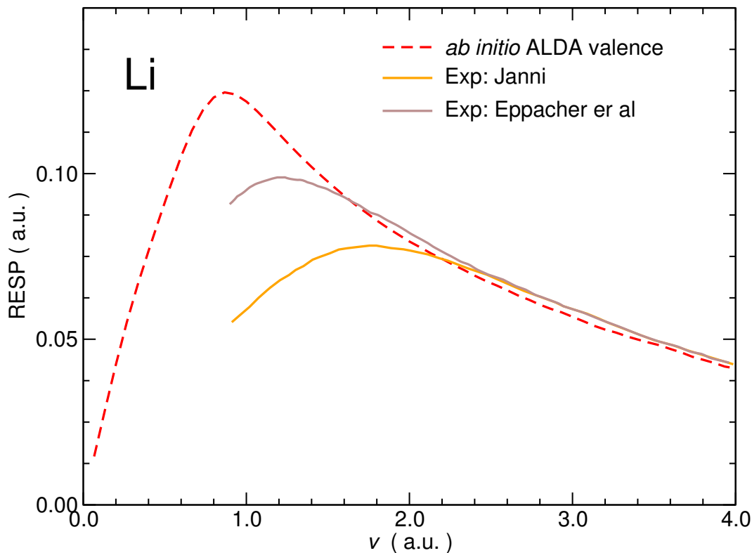
Figure 7.6: The electrons RESP of Li within ALDA in linear-response (dashed red line) compared to the available experimental data. Experiments (probably bcc crystal) by Janni [42] (orange line) and Eppacher et al. [28] (brown line).
