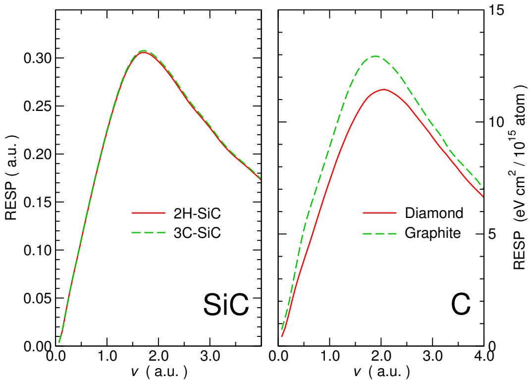
Figure 7.10: RESP of SiC (left-hand panel) and of carbon (right-hand panel) within ALDA including the 2s2p electrons of Si. 3C-SiC and 2H-SiC phases are shown for silicon carbide, whereas graphite and diamond phases are shown for carbon.
