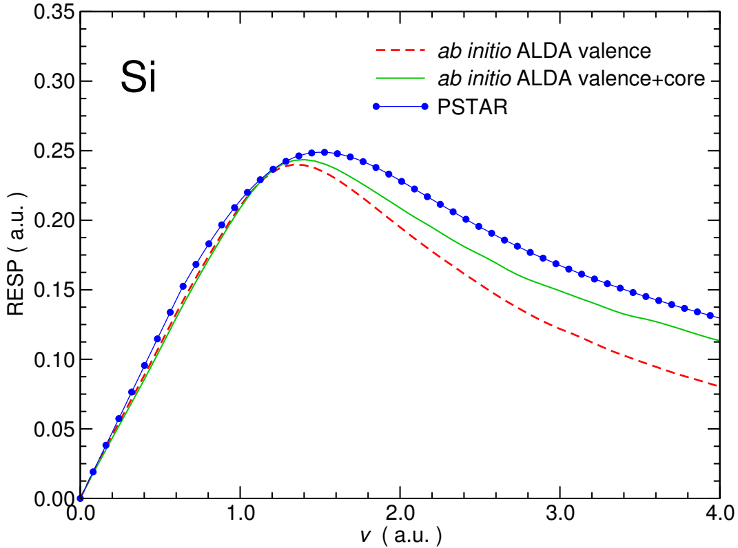
Figure 7.4: RESP of Si within ALDA including (solid green line) or not (dashed red line) the contribution from the core 2s and 2p electrons. Experiment from the PSTAR database[7] (blue circle symbols) is given as a reference.
