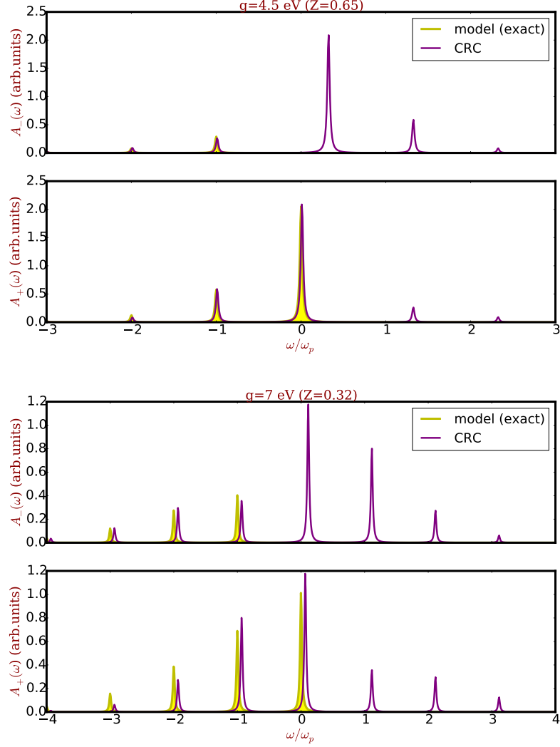
Figure 5.5: The spectral functions of the two-level hole-plasmon coupling Hamiltonian. All parameters are the same as in Fig. 5.3. Upper panel (two figures): the coupling g = 4.5 eV yielding \mathbf{Z} = 0.65 . Lower panel (two figure): a stronger coupling g = 7 eV yielding \mathbf{Z} = 0.32 . Yellow filled and purple curves are the exact and CRC spectral functions (Eq. (5.17)), respectively. The Lorentzian broadening \eta = 0.1 eV has been used for all plots.
