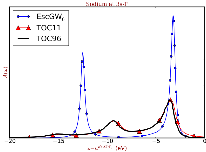
Figure 6.4: Intrinsic spectra of Na 3s at the \Gamma point. The blue curve with circles, red curve with up-triangles and black curve are intrinsic spectra of the \text{EscGW}_0 , TOC11 and TOC96 (reproduced from Ref. [9]), respectively. The zero of the energy axis is set to be the \text{EscGW}_0 Fermi energy. There is no additional broadening of spectra in this plot. The QP weight of the TOC96 has been aligned according to the QP weight of the TOC11 for good comparison.
