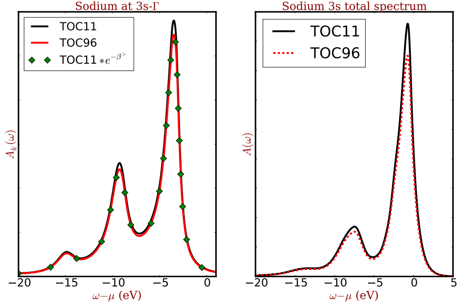
Figure 6.6: Intrinsic spectra of Na 3s. Left panel: k -resolved spectrum at the \Gamma point. Right panel: total k -summed spectrum. The black and red curves (red dashed in the right panel) are the spectra of the TOC11 and TOC96, respectively. The green diamonds in the left panel shows A^{C11}e^{-\beta} that is supposed to be the same as A^{C96} from our derivation. Our cumulant code gives indeed what we have expected in sodium valence calculation. The plots in the right panel have Gaussian broadening of 0.3 eV because they are the k -summed total spectra.
