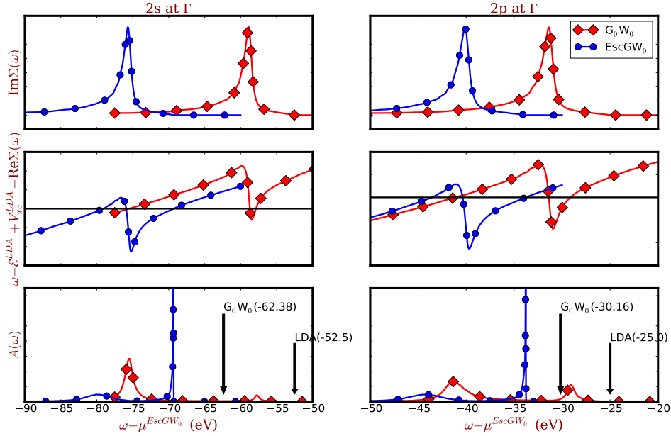
Figure 2.8: Intrinsic spectral function of the sodium 2s state at the \Gamma point (lower panel). Red curves with diamonds are G_0W_0 results, blue curves with circles are EscGW_0 results. The position of the LDA band at \Gamma is given by the black arrow labeled LDA. The arrow labeled G_0W_0 indicates the quasi-particle energy that one would obtain by the usual first-order approximation based on a linearization of the self-energy as discussed in equation (2.44). The upper two panels show the imaginary and shifted real parts of the GW self-energy. The zero of the energy axis is set to be the EscGW_0 Fermi energy.
