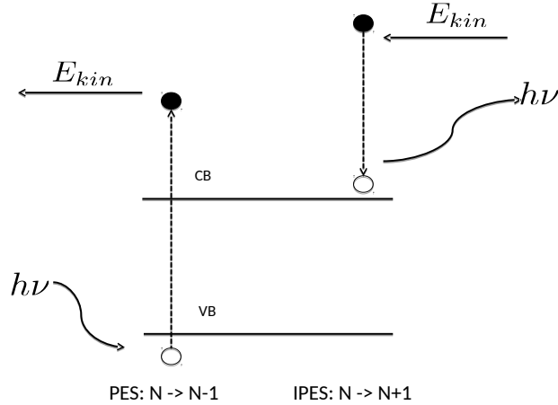
Figure 1.1: Schematic view of direct (on the left) and inverse (one the right) photoemission spectroscopy. The Fermi energy is between the valence (VB) and conduction (CB) band. In PES an electron is emitted with energy E_{kin} due to the excitation induced by the photon of energy h\nu . The IPES is the inverse process of PES where one electron is added to the system and one photon is emitted as Bremsstrahlung. In both processes we can measure E_{kin} and h\nu from which we can access the energy levels of the system using the energy conservation rule. The total number of electrons in the sample has been changed (from N to N \pm 1 ) in both processes. This is the reason why the excitations in (I)PES are called charged excitations, as opposed to the neutral excitations (e.g., excitons and plasmons) where the number of electrons is conserved during the excitation.
