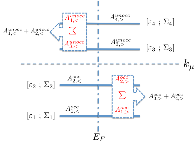
Figure 5.6: A schematic illustration of the four-level system. The states \epsilon_1 and \epsilon_2 are below the chemical potential \mu , \epsilon_3 and \epsilon_4 are states above the chemical potential. The self-energy of each state is \Sigma_i . The electron removal spectral functions of the occupied states (below the chemical potential) are A_{1,<}^{occ} and A_{2,<}^{occ} . The electron addition spectral functions of the unoccupied states (above the chemical potential) are A_{3,>}^{unocc} and A_{4,>}^{unocc} . The total electron removal spectrum of the unoccupied states are A_{1,<}^{unocc} + A_{2,<}^{unocc} , which equals to the sum of electron removal spectrum of each unoccupied state A_{3,<}^{unocc} + A_{4,<}^{unocc} , however the individual spectrum of A_{3(4),<}^{unocc} (in red color) cannot be obtained by the constrained retarded cumulant. Analogously the total electron addition spectrum of the occupied states A_{1,>}^{occ} + A_{2,>}^{occ} equals A_{3,>}^{occ} + A_{4,>}^{occ} but the individual spectrum of A_{1(2),>}^{occ} (in red color) is missing.
