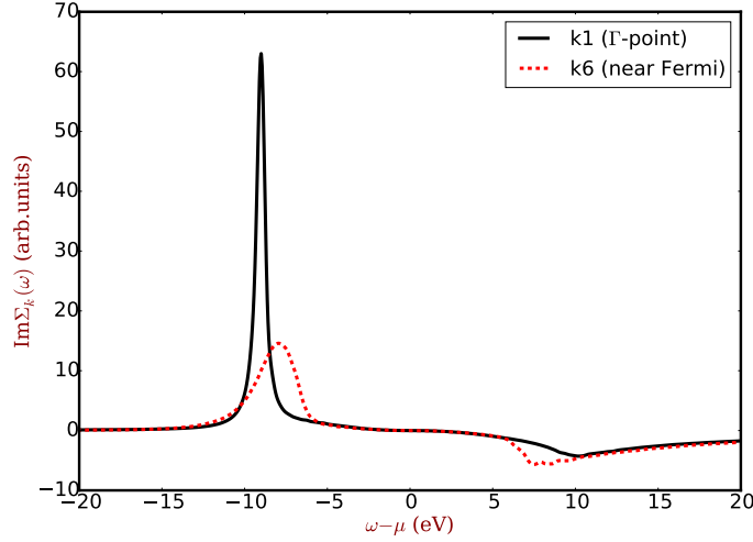
Figure 6.8: The imaginary part of the GW self-energy \text{Im}\Sigma at k_1 = [0, 0, 0] , i.e. \Gamma point (black curve) and at k_6 = [0.3125, 0, 0] , i.e. a state closer to the Fermi than \Gamma .
