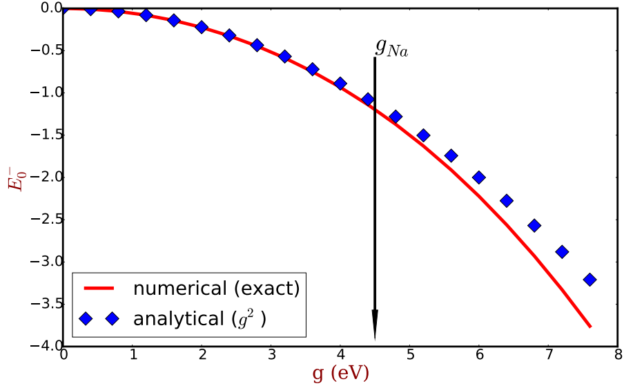
Figure 5.1: The performance of the second order expansion of the ground state energy in equation (5.1). The parameters are corresponding to bulk sodium bottom valence state, i.e. \epsilon_0 = \mathbf{t} = 1.5 eV and \omega_p = 6 eV. Red curve is the exact numerical total energy E_0^- and blue diamonds are the total energy calculated from the second order expansion in Eq. (5.1). In particular, g = 4.5 eV (black arrow labeled “ g_{Na} ”) corresponds to the sodium case where the error of the second order expansion is about 6%. This figure shows that Eq. (5.1) is a sufficiently good approximation to the exact total energy of the HPC-2.
