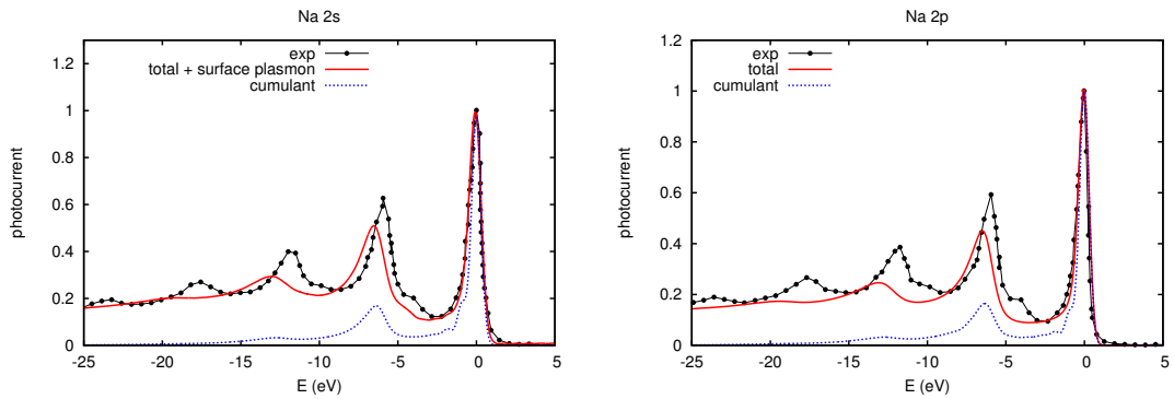
Figure 6.2: Comparison of the experimental photoemission spectrum to the spectrum calculated using the TOC11 + extrinsic + interference approach: Left, Na 2s ; right: Na 2p . The red solid lines are total calculations, including secondary electron background, black with circles are experimental data [47], and blue dashed are calculated TOC11 intrinsic spectral functions. The total Na 2s calculated spectrum also includes an approximation to the surface plasmon contribution. The spectra are angle-integrated. Original experimental data were in arbitrary units: here we have normalized them to the main-peak intensities. The calculated QP energies have been aligned with respect to the experimental QP peaks otherwise the GWA 2s level is too deep by about 5 eV, and the 2p level by about 3 eV (see table 2.1). The zero of the energy axis is set to be the QP energy of the experiment. Gaussian broadening of 0.3 eV has been used in all calculated spectra. The extrinsic and interference effects have been calculated by my co-author J. Kas and J. Rehr in Ref. [20].
